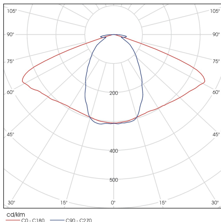
Industrial LED luminaire LED 120, 5000K
