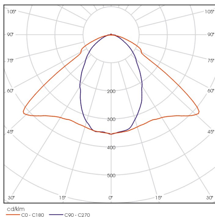
Industrial LED luminaire LED 96, 5000K, with diaphragm
