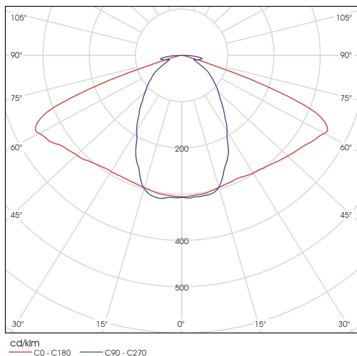
Industrial LED luminaire LED 72, 5000K
