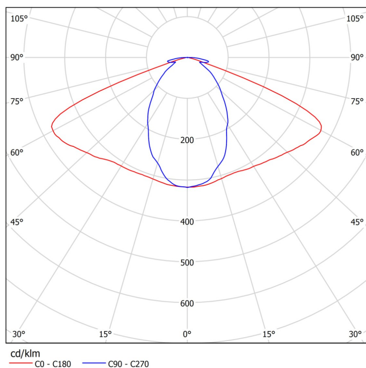
Industrial LED luminaire LED 96, 5000K
