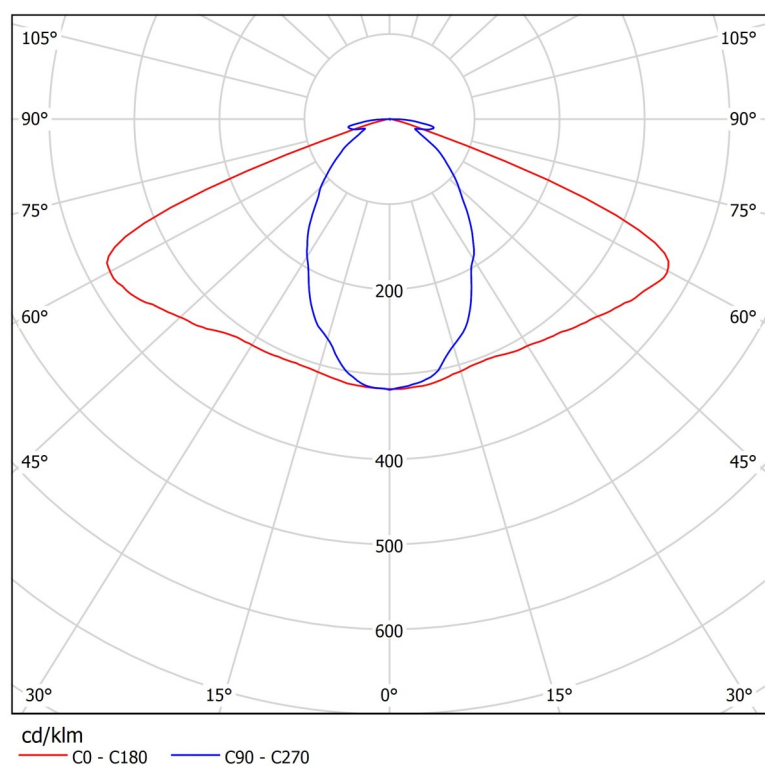
Industrial LED luminaire LED 144, 5000K
