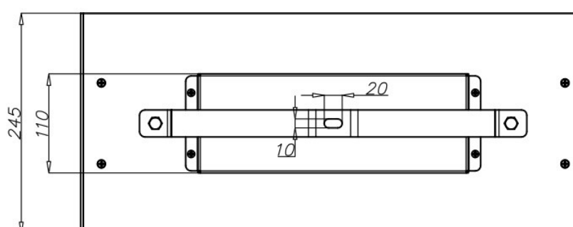
Industrial LED luminaire 96, 120, 144
