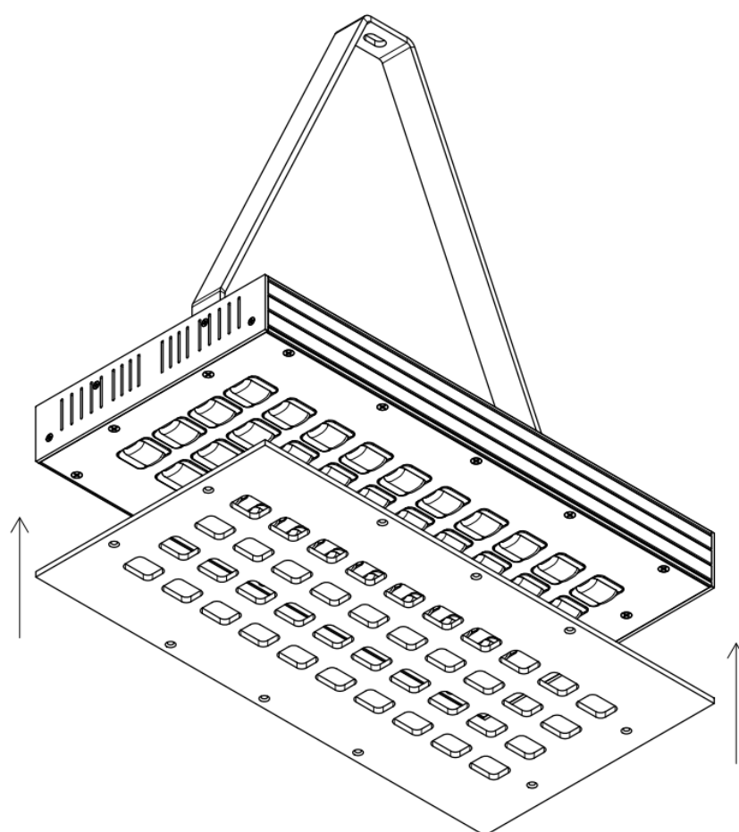
Assembly of diaphragm
