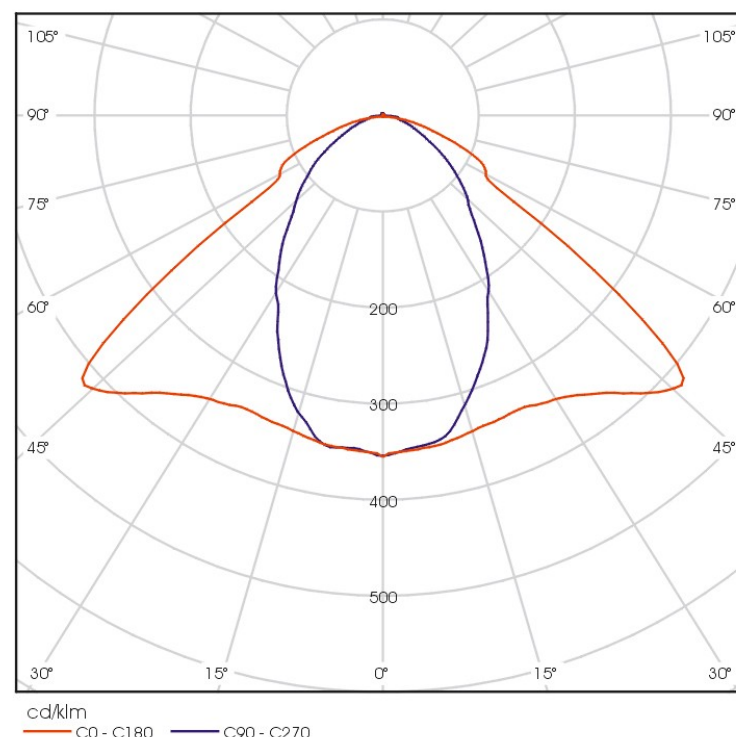
Industrial LED luminaire LED 120, 5000K, with diaphragm
