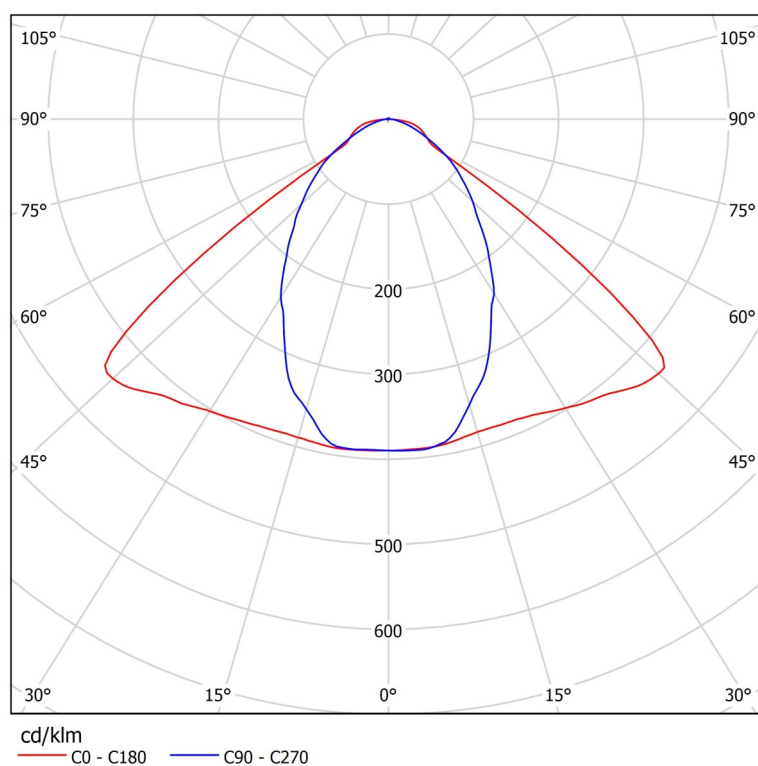
Industrial LED luminaire LED 144, 5000K, with diaphragm
