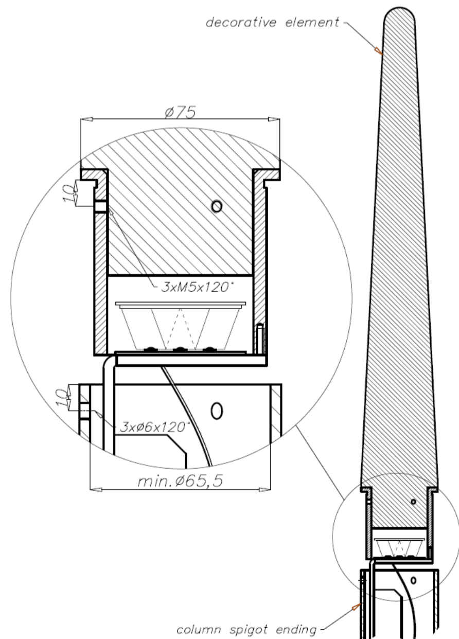
Way of mounting on the column spigot ending
