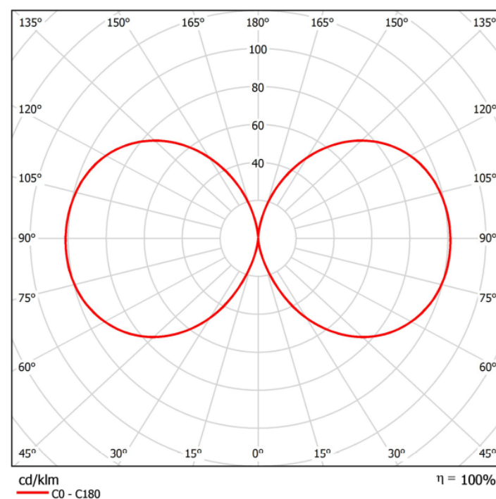
Distribution curve SAL DECO-3 LED
