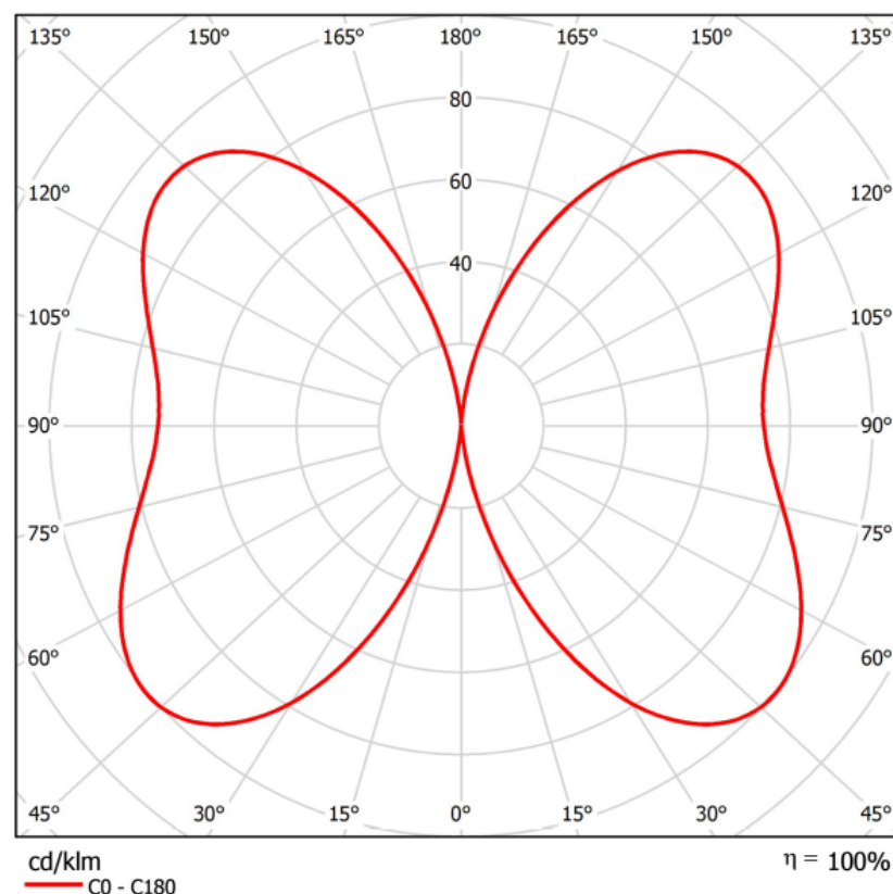
Distribution curve KARIN DECOR 2400 LED
